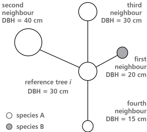
FIGURE 2 A structural group of four for calculating the species mingling and the DBH differentiation index (Pommerening [15] modified after Albert and Gadow [17])
